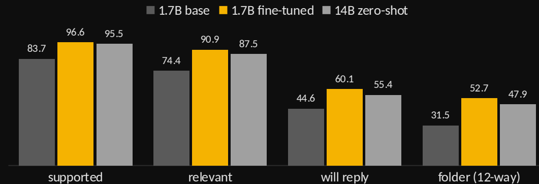
Held-out accuracy, %
